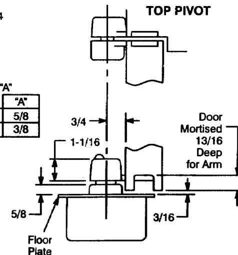
WITH FLOOR PLATE Set Cement Case Flush with Surface of Finished Floor
